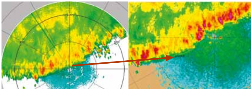
Attenuation correction illustrated. Left panel, corrected reflectivity fields at C-band, and right panel, S-band measurement at the same time. The arrow points to the C-band radar location versus S-band radar location.
