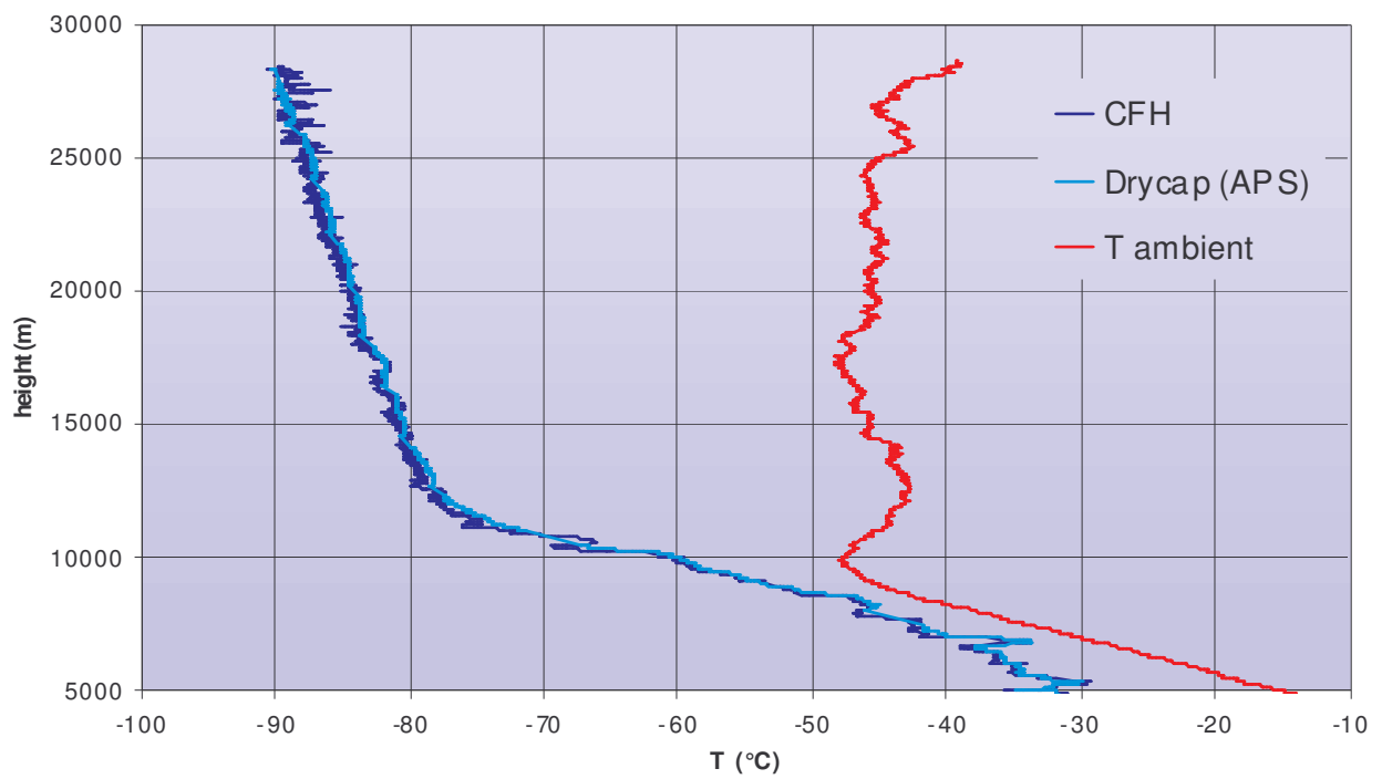
Fig 2. First test results of the DRYCAP® sensor: comparison against CFH in July 2007.
