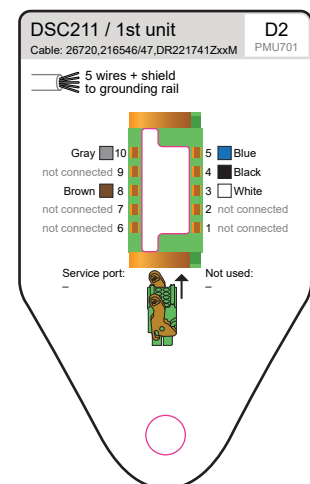
Quick reference card for sensor wiring
