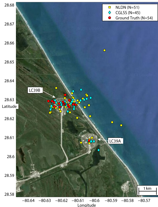
Figure 1. Ground truth, NLDN, and CGLSS strike point locations.
