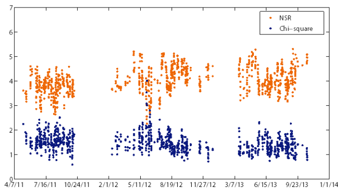
Figure 5. Time series of chi-square and NSR for the CGLSS system from May 2011-October 2013.
