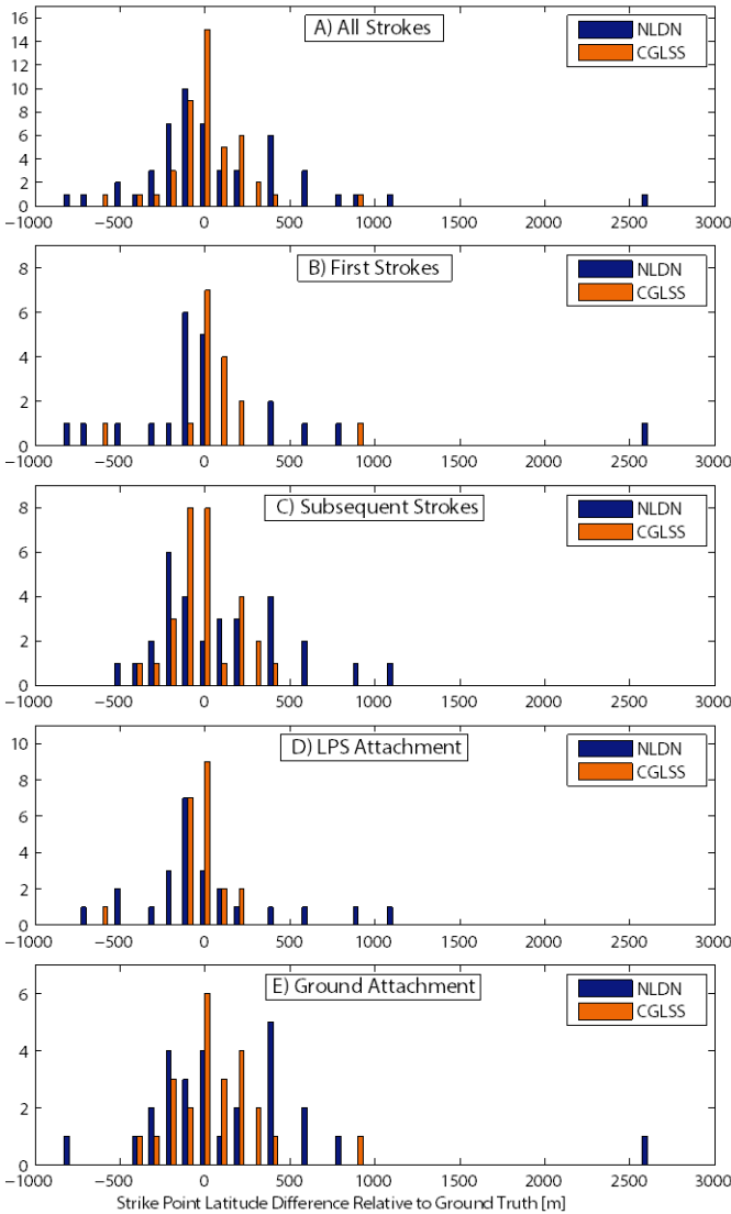
Figure 4. Distributions of latitudinal strike point location differences of NLDN and CGLSS systems relative to ground truth.
