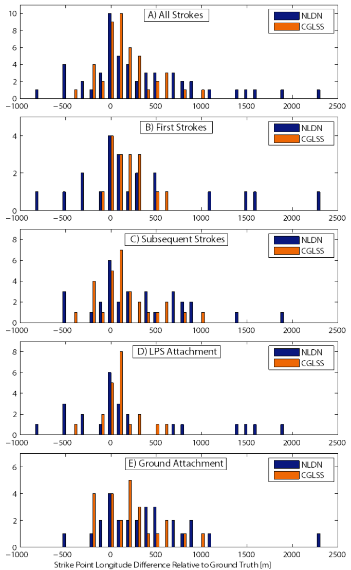
Figure 3. Distributions of longitudinal strike point location differences of NLDN and CGLSS systems relative to ground truth.
