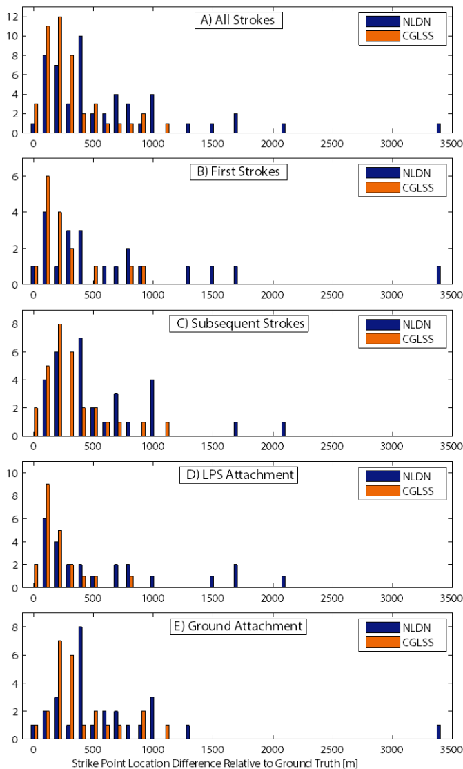
Figure 2. Distributions of strike point location differences of NLDN and CGLSS systems relative to ground truth.
