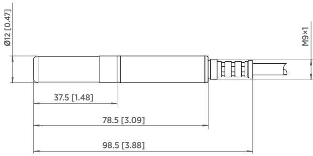
HMT313 探头
