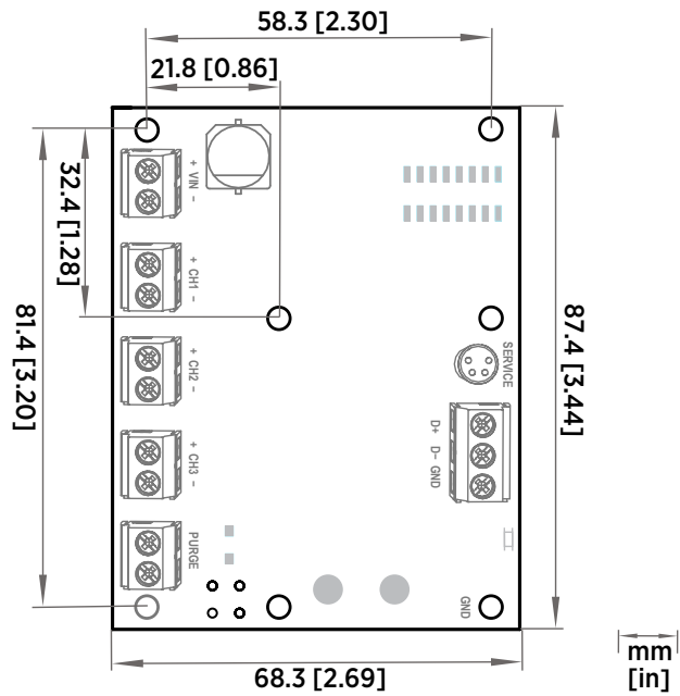
Component Board Dimensions
