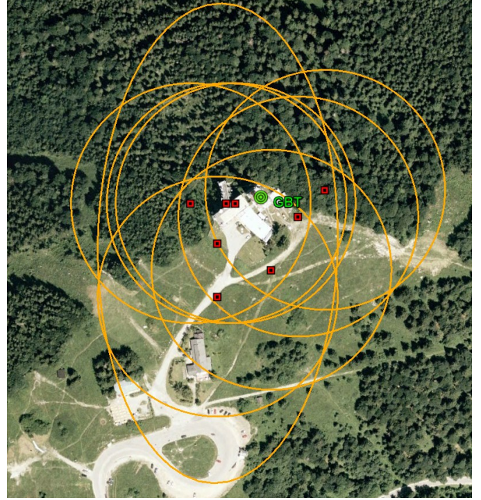
Fig. 7. Locations of 8 return strokes in GBT flash #885 from 02-06-2013 at 05:20:42 (UTC) with their assigned 50% confidence ellipse.
