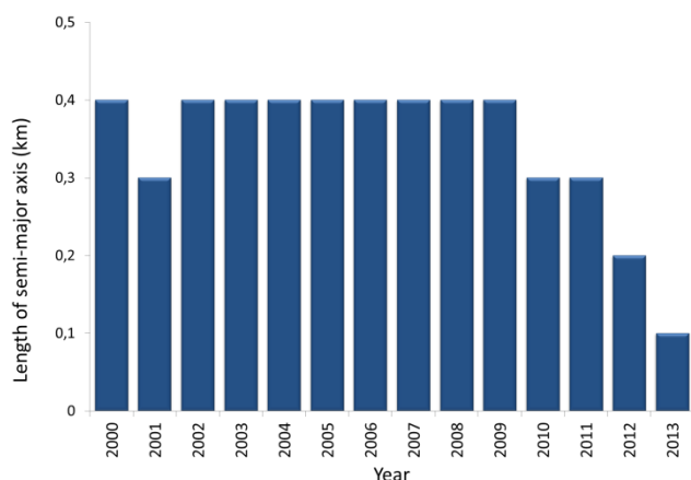
Fig. 8. Median length of semi-major axis of 50% confidence ellipse for EUCLID located negative strokes in a 100 km radius circular area in Austria centered 14.0°E/47.5°N (Calculation is based on about 100.000 Strokes per year)
