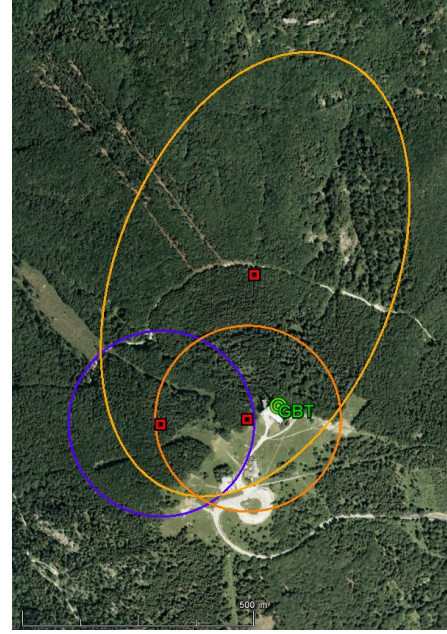
Fig. 2. ALDIS locations of 3 strokes in GBT Flash #783 (05/07/2010 08:13:16 UTC). Two confidence ellipses include the GBT site (orange line) and one ellipse does not (purple line).
