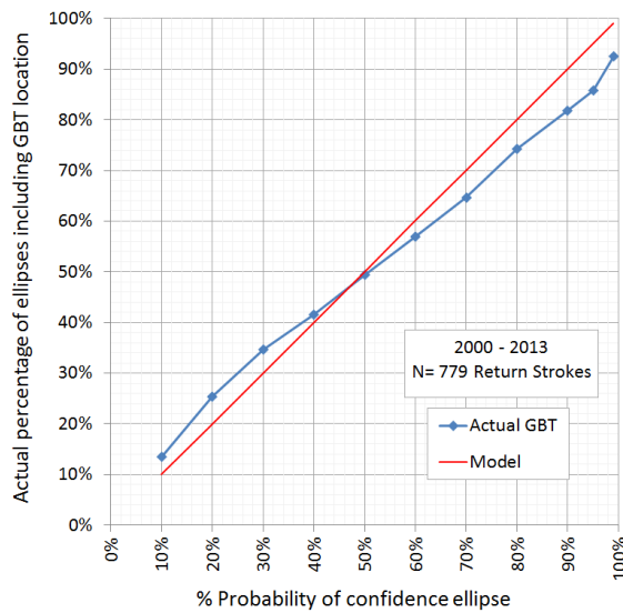
Fig. 3. Percentage of located return strokes assigned confidence ellipses that include the true GBT location.
