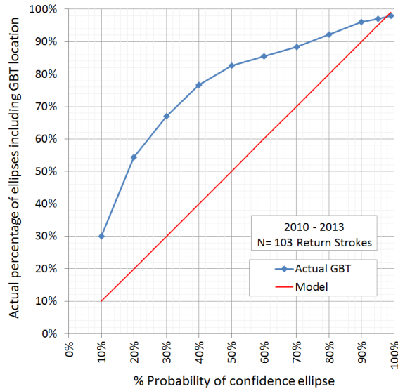
Fig. 5. Percentage of located return strokes assigned confidence ellipses that include the true GBT location for the period 2010–2013.
