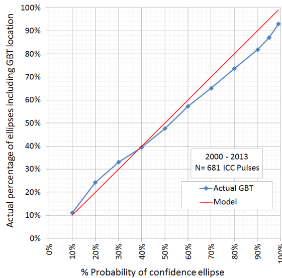
Fig. 4. Percentage of located ICC-pulses assigned confidence ellipses that include the true GBT location.
