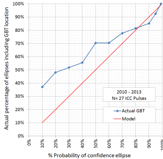
Fig. 6. Percentage of located ICC pulses assigned confidence ellipses that include the true GBT location for the period 2010–2013.
