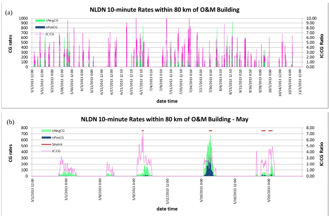
Fig. 7. NLDN Lightning observations within 80 km of the O&M building, for 10-minue periods, including negative CG stroke count (green bars), positive CG stroke count (blue bars, not easily seen), and IC:CG ratio (cloud pulses / CG strokes). (a) Full season; (b) zoom-in of same display as (a) for the periods of May 1-20. Local severe storm report periods (large hail, tornados, and high surface winds) are indicated by red bars.
