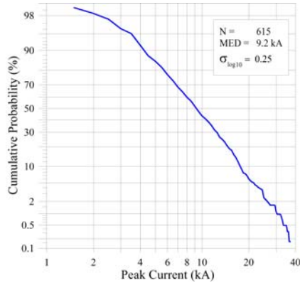
Fig.4: Distribution of the peak current of return strokes in upward initiated lightning to the GBT (2000- 2007)
