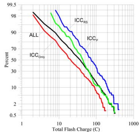
Fig.3: Cumulative frequency distribution of total charge for all negative upward flashes and the three categories ICC RS , ICC P and ICC Only at the GBT (2000 – 2007)
