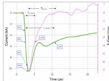
Fig.7: Current and vertical E-field waveform for GBT stroke #558-2. Current and field pulse are aligned in terms of starting point and peak amplitude (right hand side scaling applies to inverted E-field waveform) (adopted from Pichler et al., 2010)
