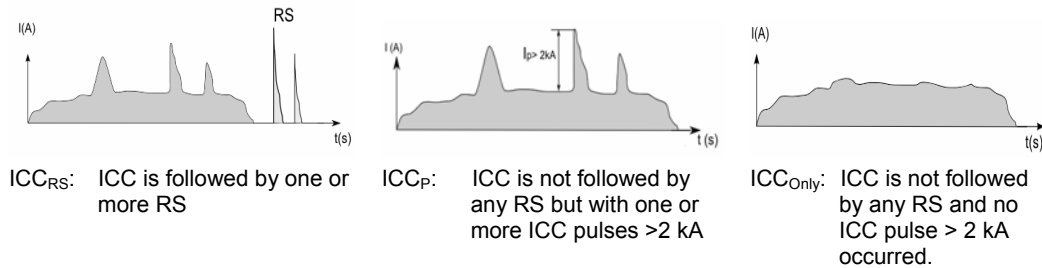
Fig.2: Schematic records of upward initiated lightning flash currents
