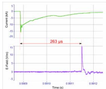
Fig.6: Current and correlated E-field measured at a distance of 78.8 km of a typical RS-pulse (pulse #554-10). I_p = -15.9 kA, E_p = +15 V/m (according to the "atmospheric electricity sign convention" a negative stroke produces a positive E-field pulse)
