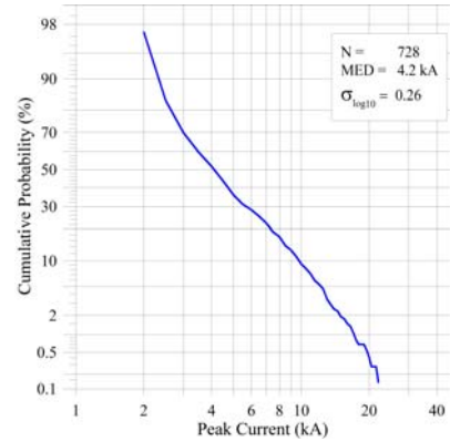
Fig.5: Distribution of the peak current of ICC-pulses in upward initiated lightning to the GBT (2000- 2007)
