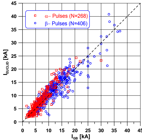
Fig.10: EUCLID peak currents plotted versus peak currents measured at the GBT during the season 2000–2005.
