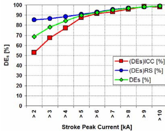
Fig.8: Stroke DE S as a function of minimum peak current
