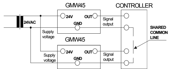
Connection of one AC supply to several transmitters
