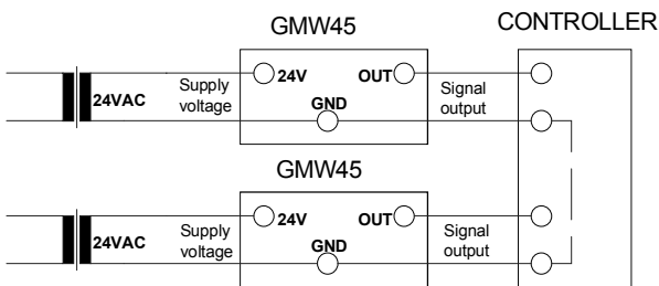
Connection of separate AC supplies (recommended)
