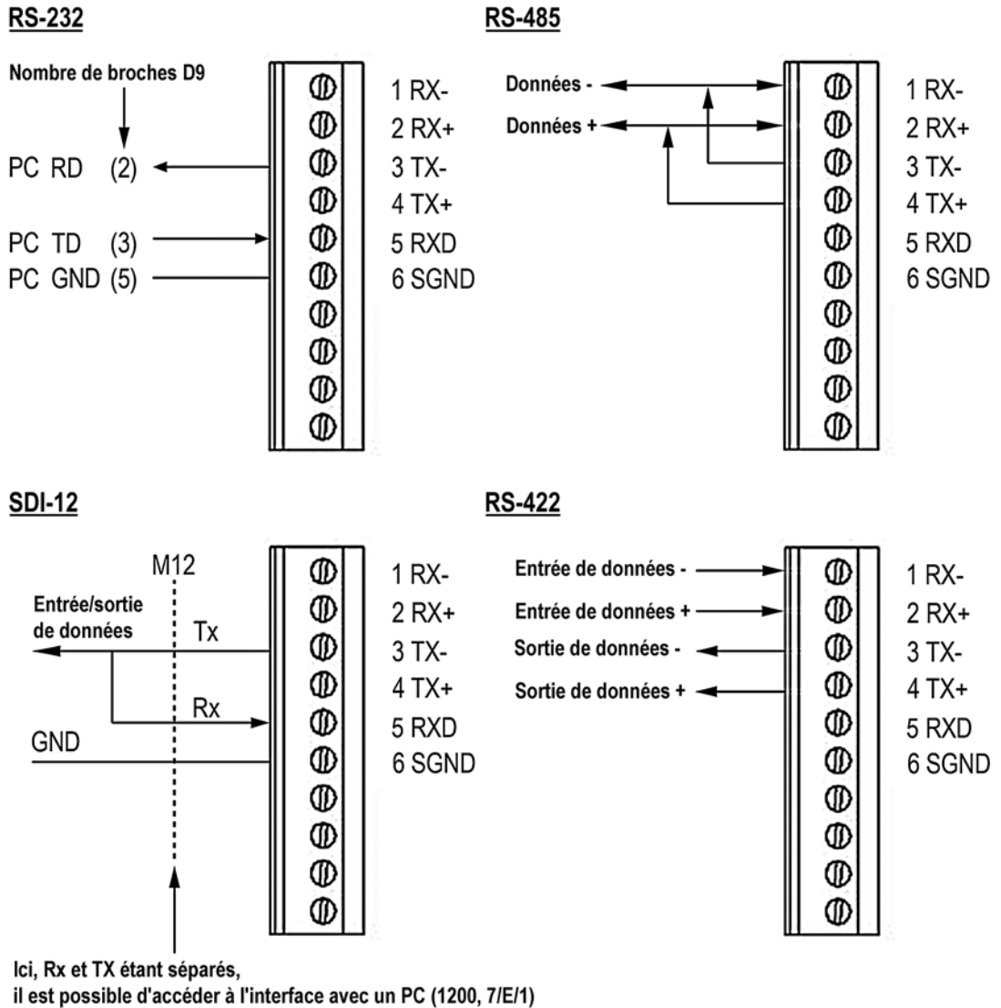
Figure 25 Interfaces de communication
