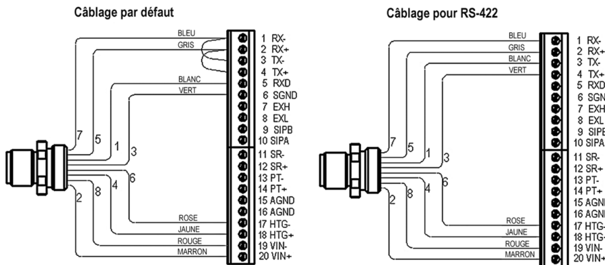
Figure 23 Câblage interne
