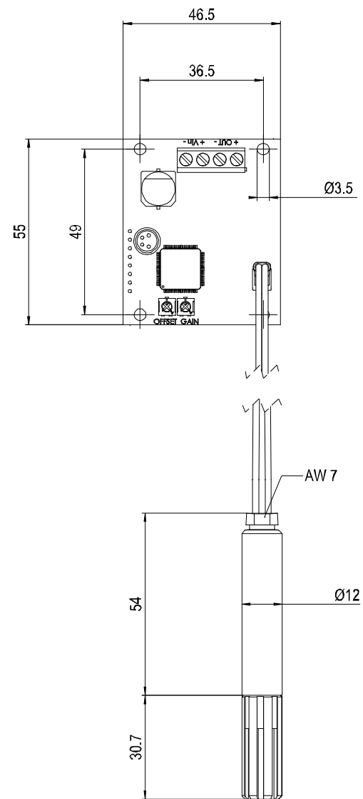
Figure 5 Dimensions in mm
