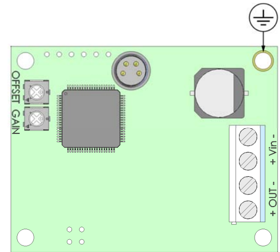
Figure 1 Component Board (3-wire version)
