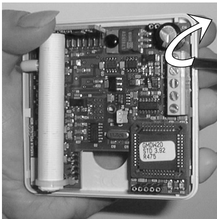
Figure 1 Cable routing
