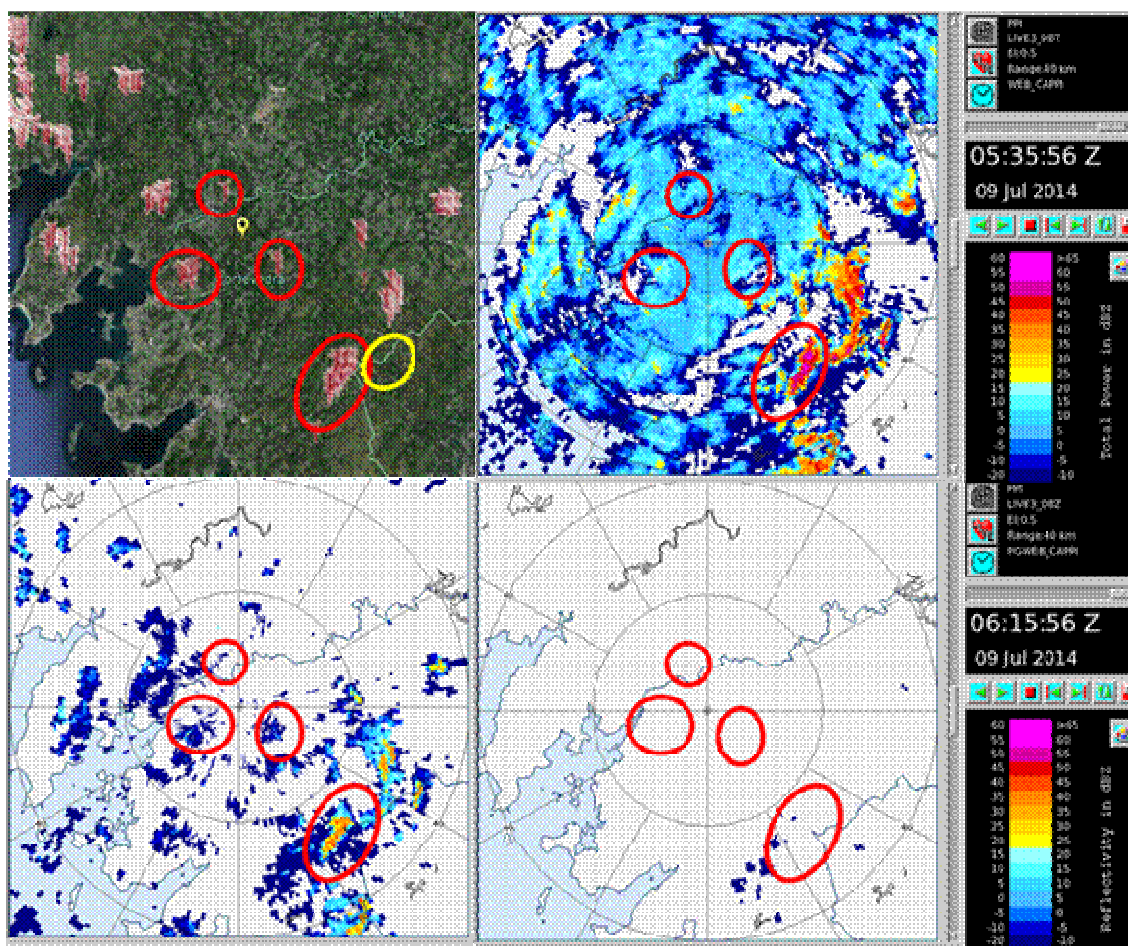
Figure 6: a) the location of verified wind turbines within the range of 40 km from the Valga radar. Red ovals indicate the sites of echo evaluation. The yellow oval marks the reference hill without turbines (plain ground echo). b) Fields of total echo in units of dBZ observed at the Valga radar. c) Fields of Doppler filtered reflectivity. In b) and c) LOG censoring is applied at P/N=1.2 dB. d) Fields of reflectivity after all the quality considerations, see Section 5.
