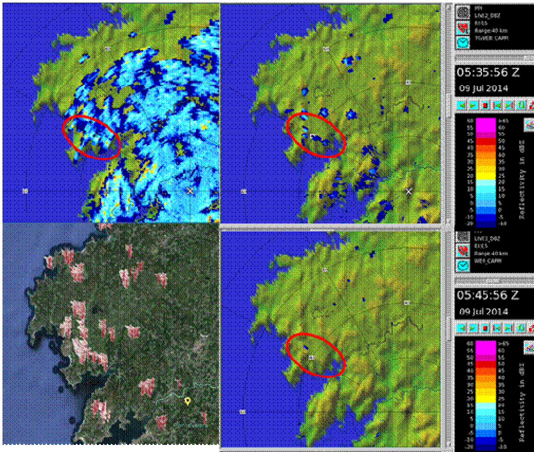
Figure 15: A region of wind farm clusters. a) total echo, b) field of Doppler filtered reflectivity subject quality considerations in clear air conditions, see text. c) locations of wind farms, and d) field of Doppler filtered reflectivity subject quality considerations in wide spread precipitation, see text.
