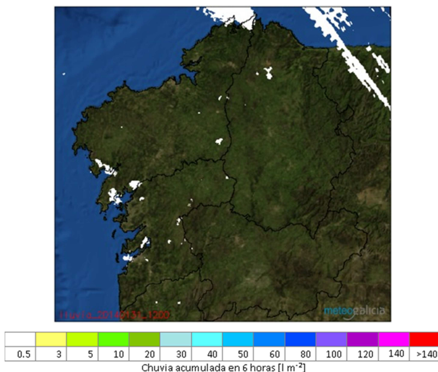
Figure 16; the public report of six hours of rain fall accumulation on the January 31 st (06-12 UTC) computed from the reflectivity scans in the precipitation mode while fair weather dominates most of the onshore area within Galicia.
