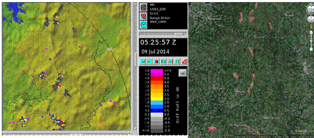
Figure 5; Recognition of wind farm locations by the Valga WRM200 radar. On the left, the fields of Doppler filtered differential reflectivity. They are censored at P/N=1.2 dB. The bins of negative differential reflectivity associate closely with the locations of wind turbines visualized on the right. An exception relate with an active construction site of other type. The turbine locations are obtained from independent data base and they have been verified in the GoogleEarth imagery,
