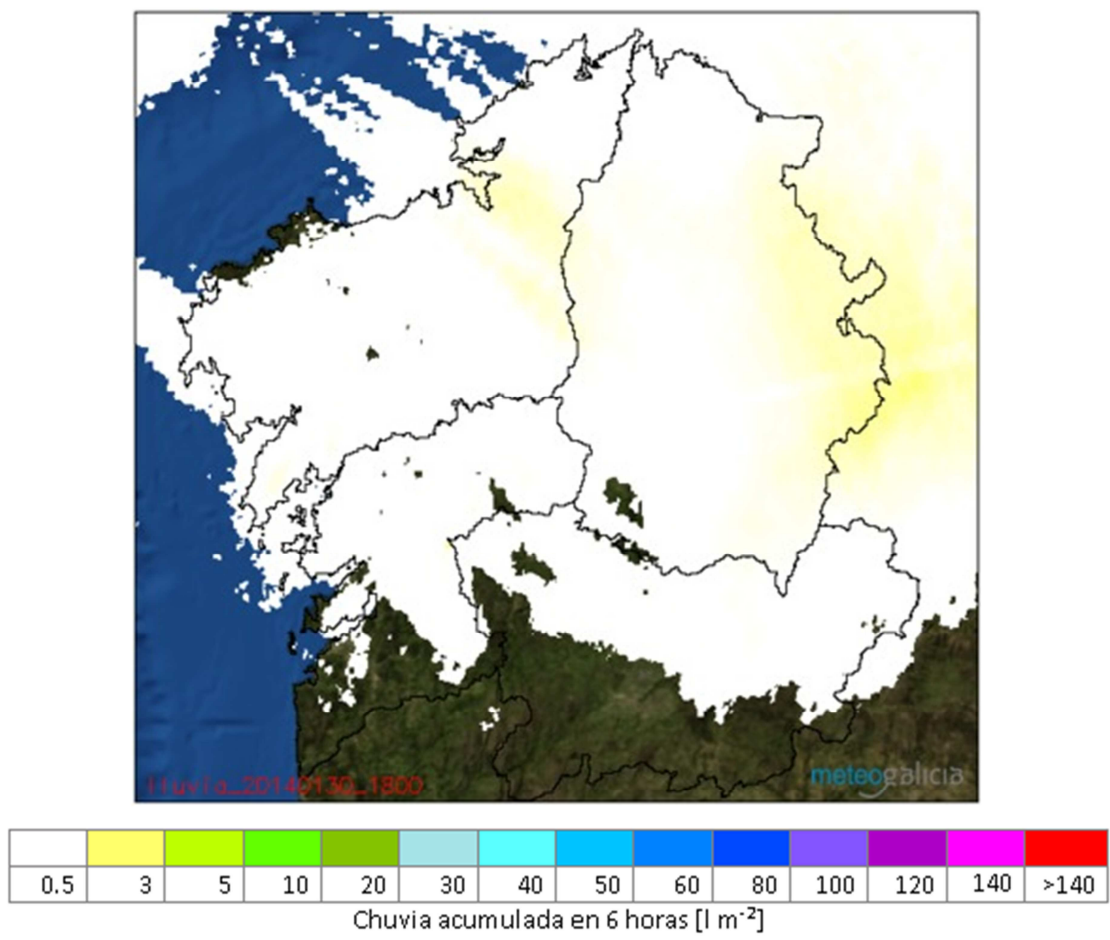
Figure 17; the public report of six hours of rain fall accumulation on the January 31 st (12-18 UTC) computed from the reflectivity scans when precipitation passes through Galicia from North towards South.
