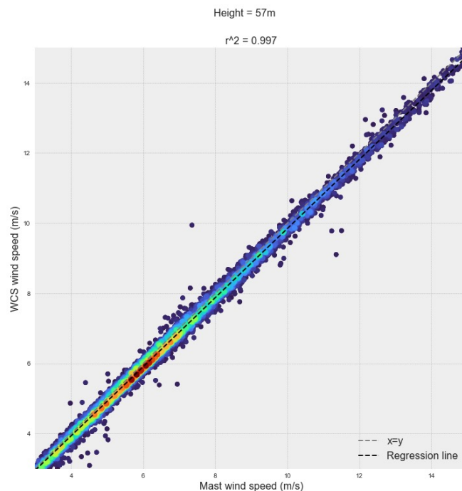
Wind speed measurement comparison of WindCube Scan and met mast.
