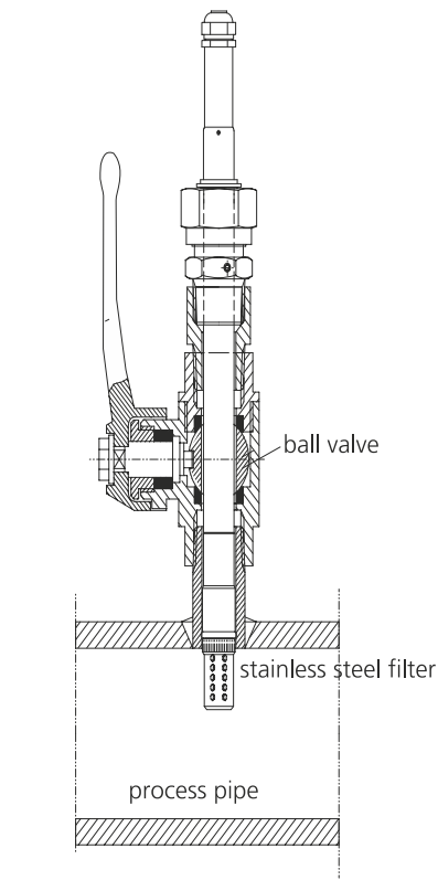
Figure 3: A ball valve installation in a process pipe line.
